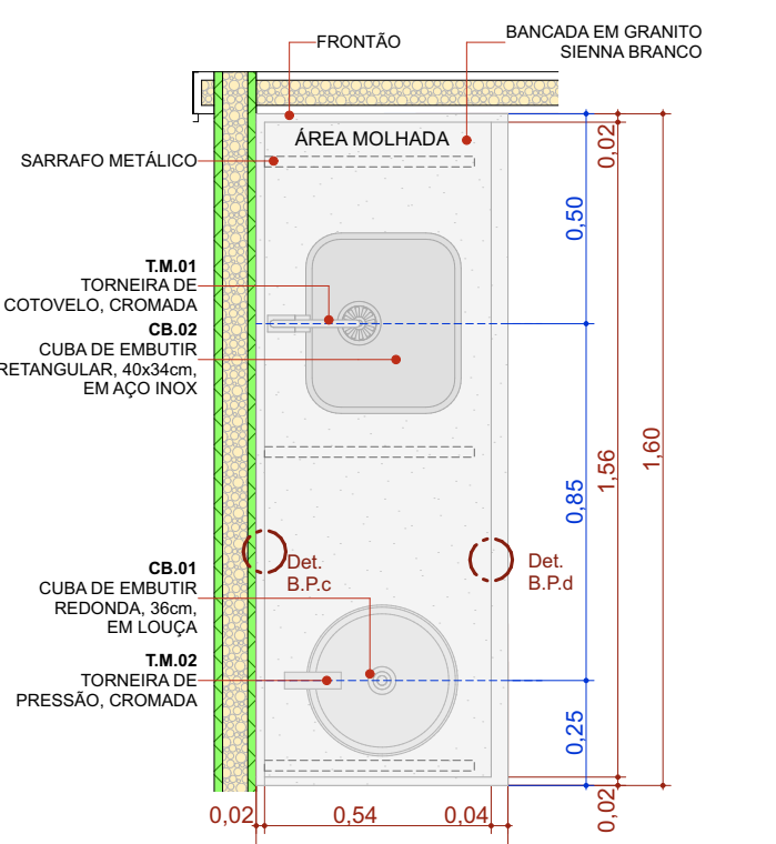
BPC.160d Escala:1:20
