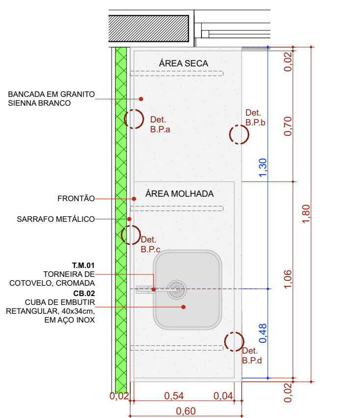
BPC.180d Escala:1:20
